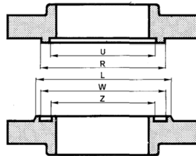
INCAMERATURA DOPPIA LARGA LARGE TONGUE AND GROOVE
